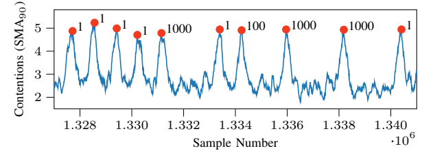
(b) Cross-VM. The absolute height of the peaks, which corresponds to the number of scheduler contentions, is approximately 10 % of those in the cross-process scenario.
