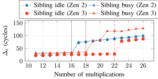
Figure 5: Effect of an empty loop on the sibling thread on the average timing differences on Zen 2 and Zen 3 ( n = 100\,000 ).
